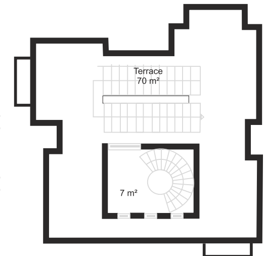
ROOF FLOOR PLAN
